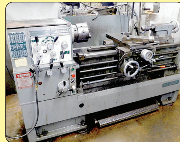
Millport Model SJ-1640G Tool Room Lathe
