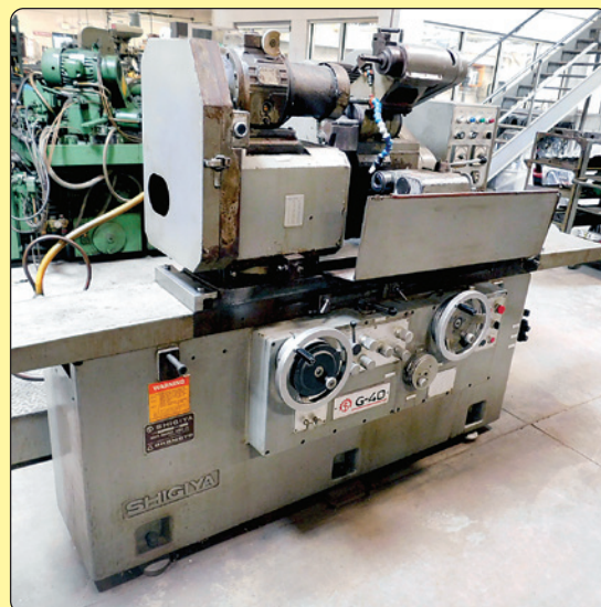
Shigiya Model GUA-40-60 Universal Cylindrical Grinder
