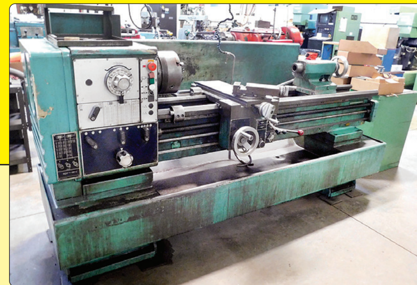
Harrison 17"x60" Engine Lathe
