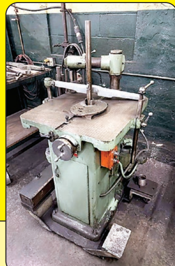
D.C. Morrison Model K Keyseater
