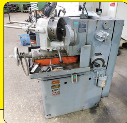
Oliver of Adrian Model DT Drill Grinder
