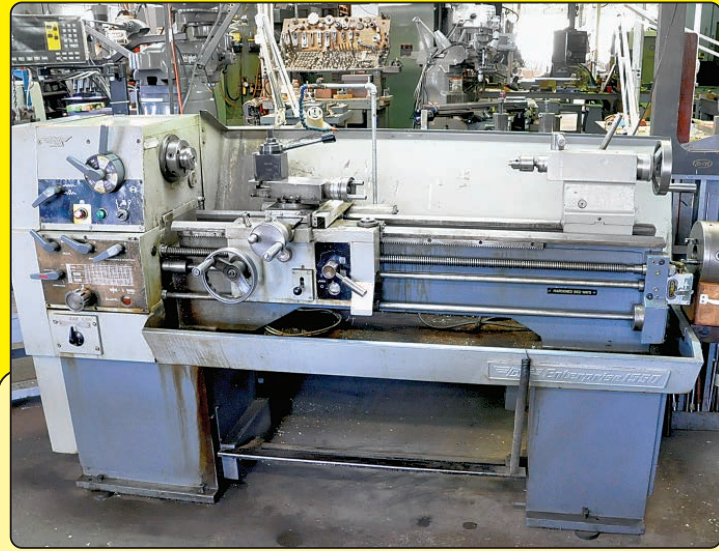
Enterprise 15" X 50" Engine Lathe
