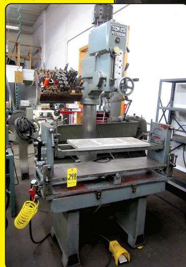
Peterson Model TCM-25 Valve Guide and Seat Machine
